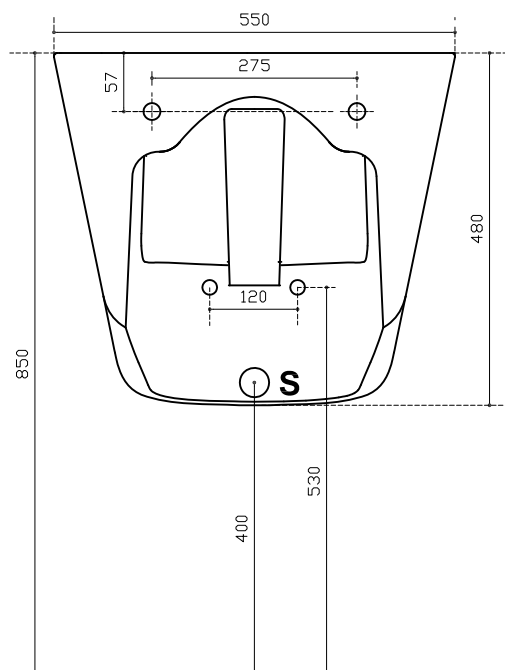
Vista posteriore Rear View
