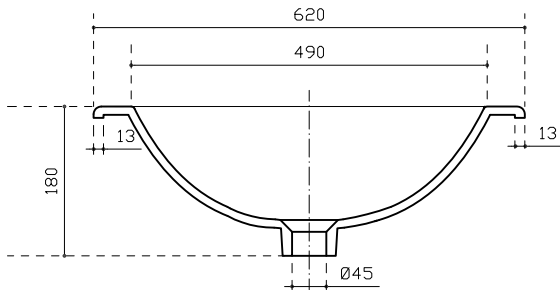
Vista frontale Frontal View Vista frontal Vue frontale
